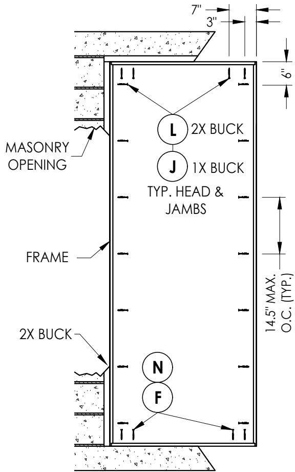
FRAME ANCHORING Masonry construction
