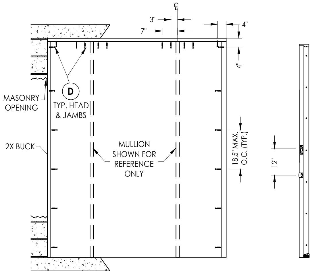
BUCK ANCHORING
