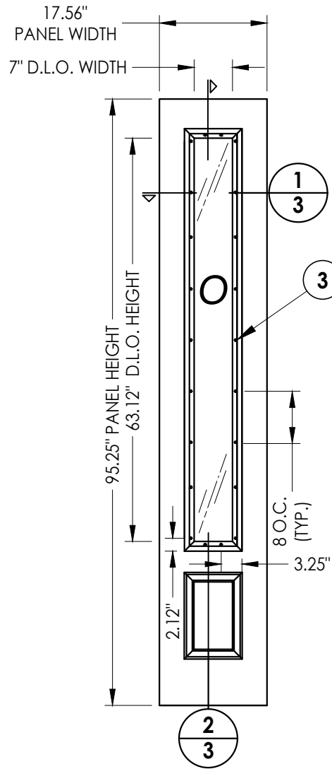
50 SIDELITE PANEL Fiberglass
