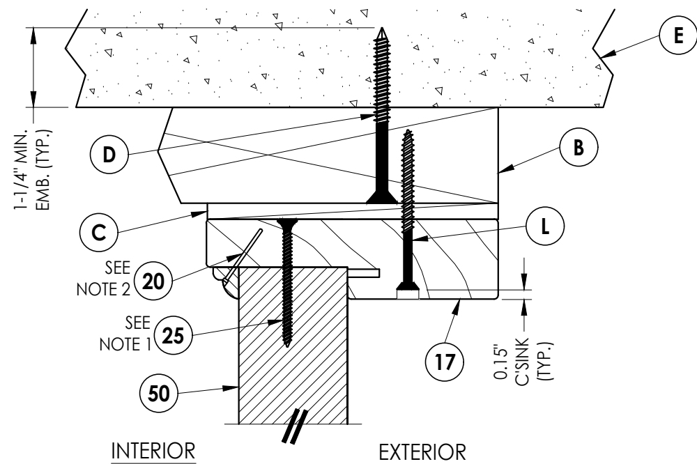
1 VERTICAL CROSS SECTION 8 Inswing shown - outswing also approved
