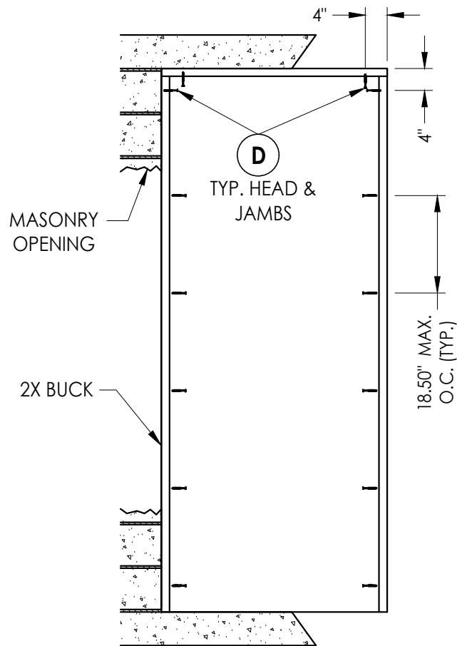
BUCK ANCHORING
