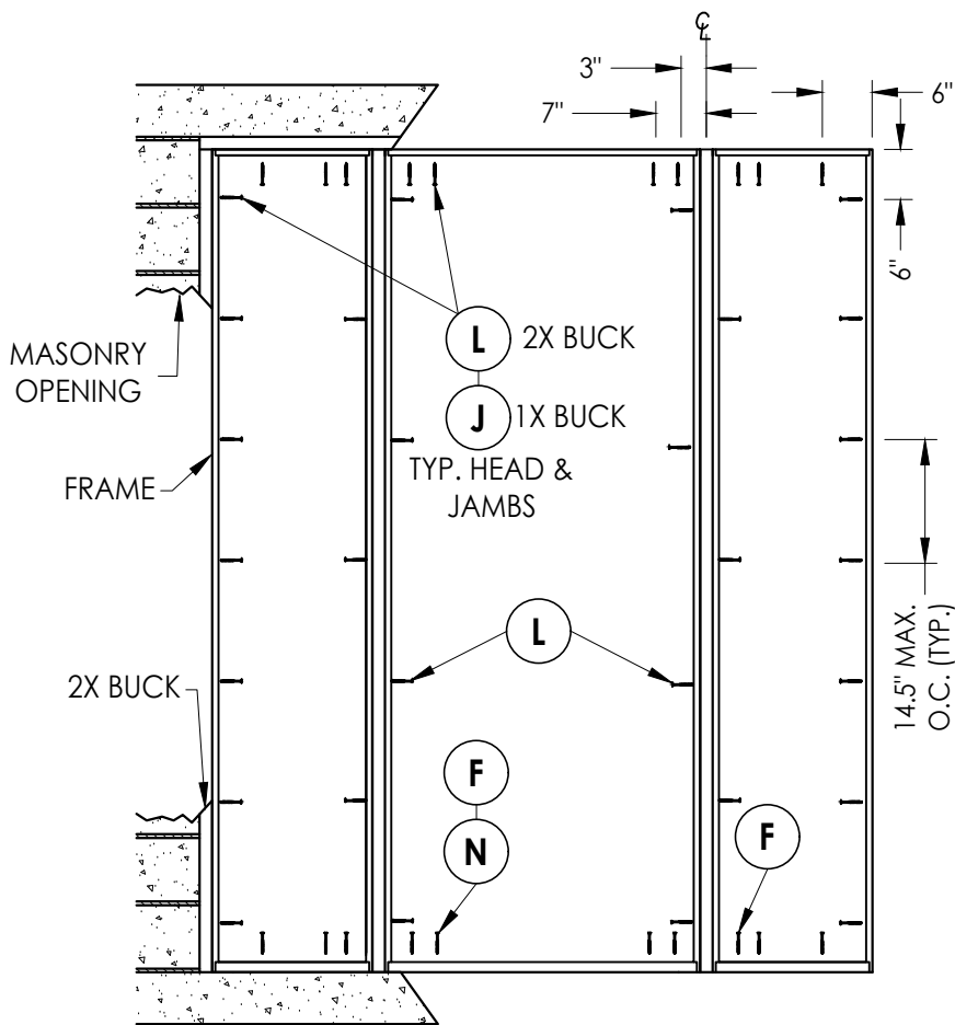
FRAME ANCHORING Masonry construction
