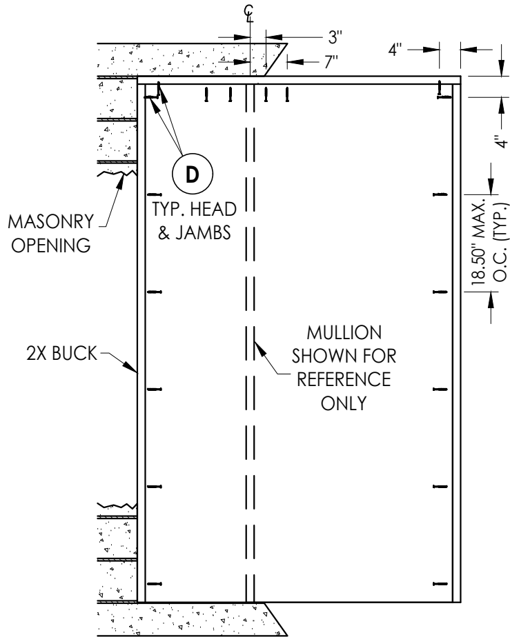
BUCK ANCHORING
