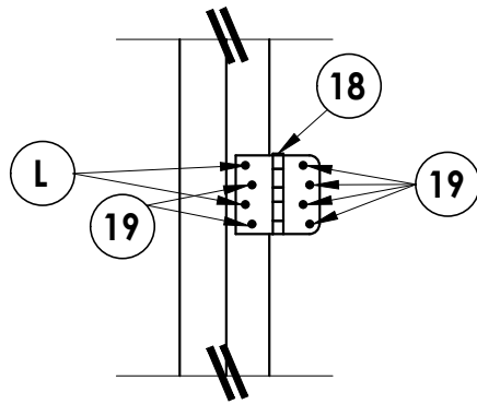
HINGE DETAIL
